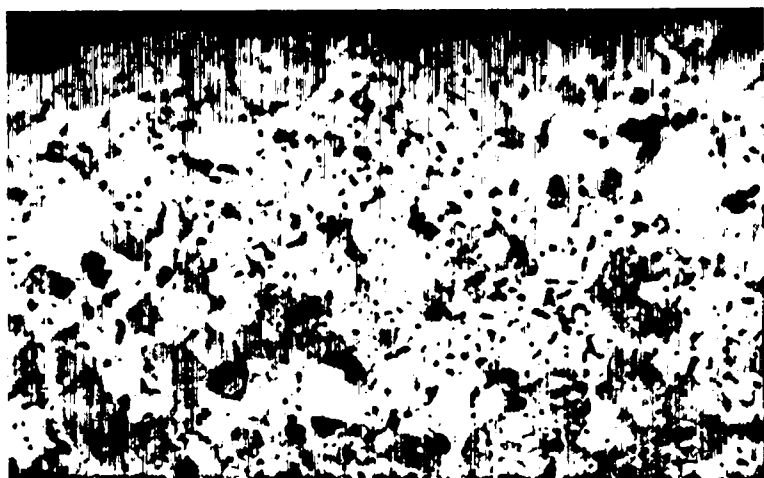
Fig. 464-7. Intergranular attack at the surface of single-phase (U,Pu)C pellet. Etched, 300X.
