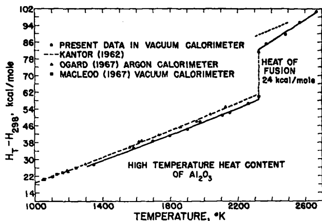
Figure 463-1. High Temperature Heat Content of \text{Al}_2\text{O}_3
