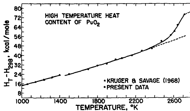
Figure 463-2. High Temperature Heat Content of \text{PuO}_2
