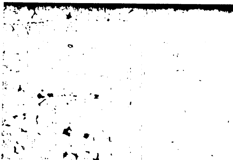
Fig. 464-5. Carburized zone on the wall of a Type 316 stainless steel capsule at junction of two single-phase carbide pellets. Etchant: 10% oxalic acid, electrolytic. 300X.
